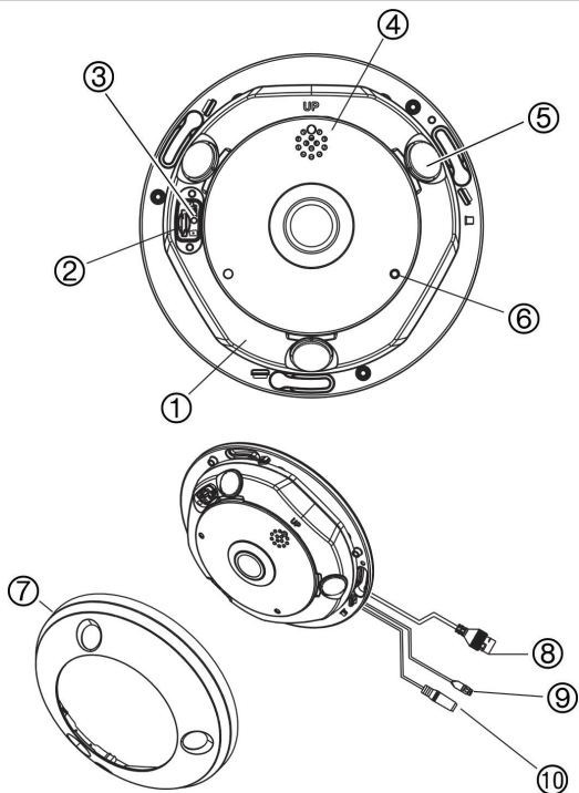
Figure 1: 360° camera
