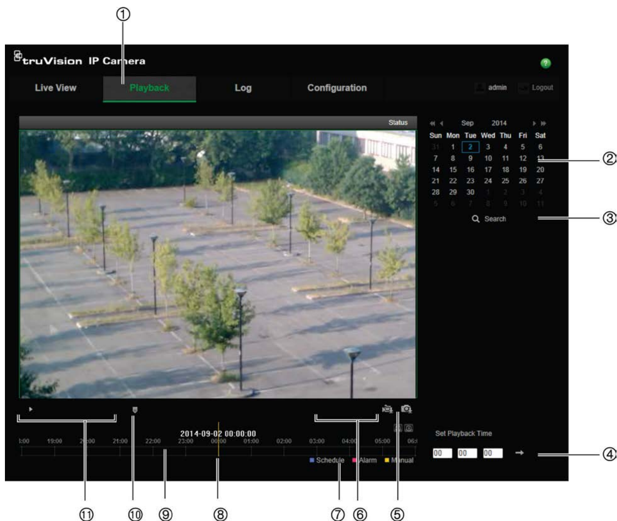
Figure 25: Playback window
