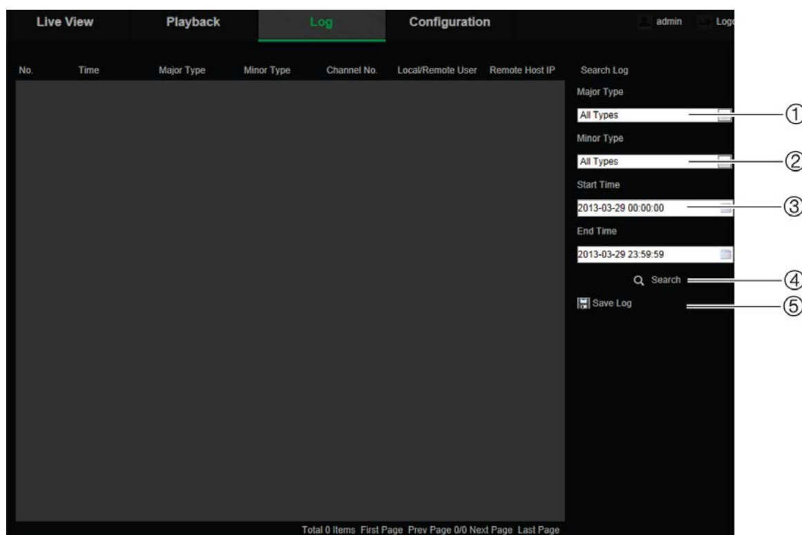
Figure 26: Log window
