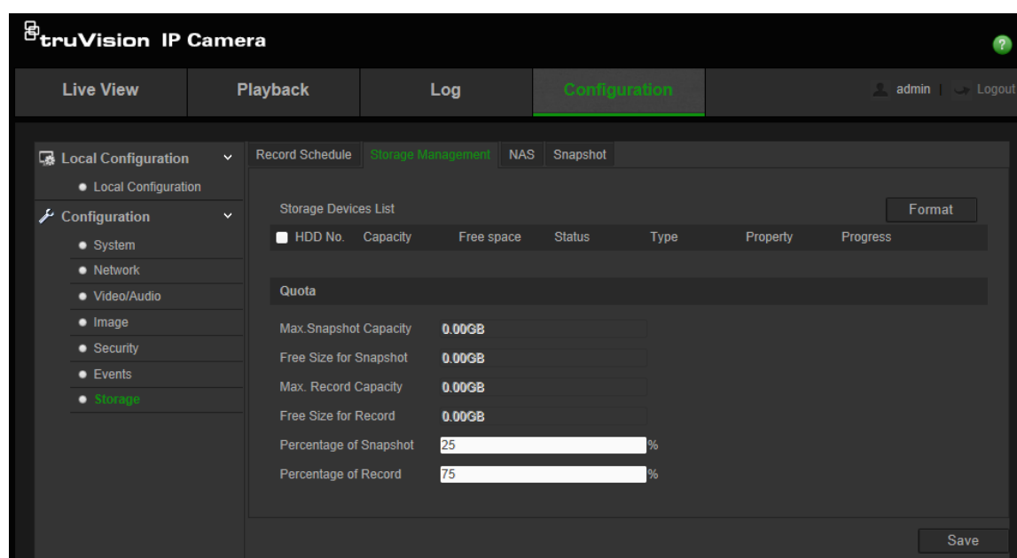
Figure 20: Storage window
